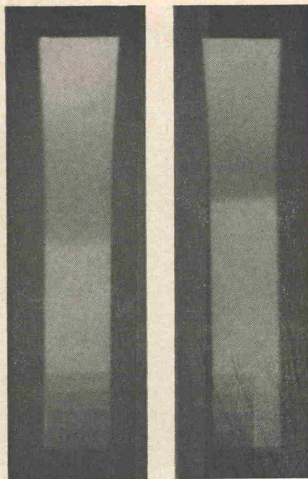
FIG. 12. Radiographs of detonation in one-dimensional channel flow for mixes G (left) and C (right). The aluminum "step wedges" are visible in the lower parts of the radiographs. The detonation is proceeding in both cases from top to bottom. The radiographs illustrate the relatively small expansion of the stream tube with this confinement.
